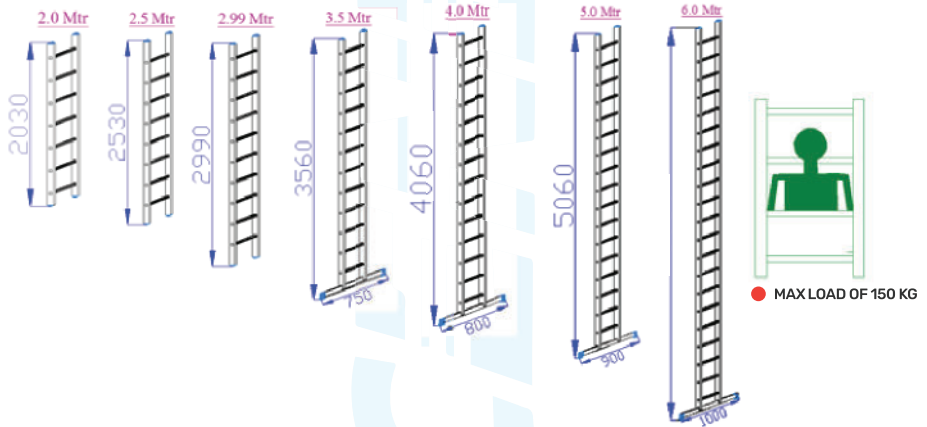
STRAIGHT / SINGLE POLE LADDER: BS EN 131-1, 2 & 3 (TECHNICAL SPECIFICATION)
